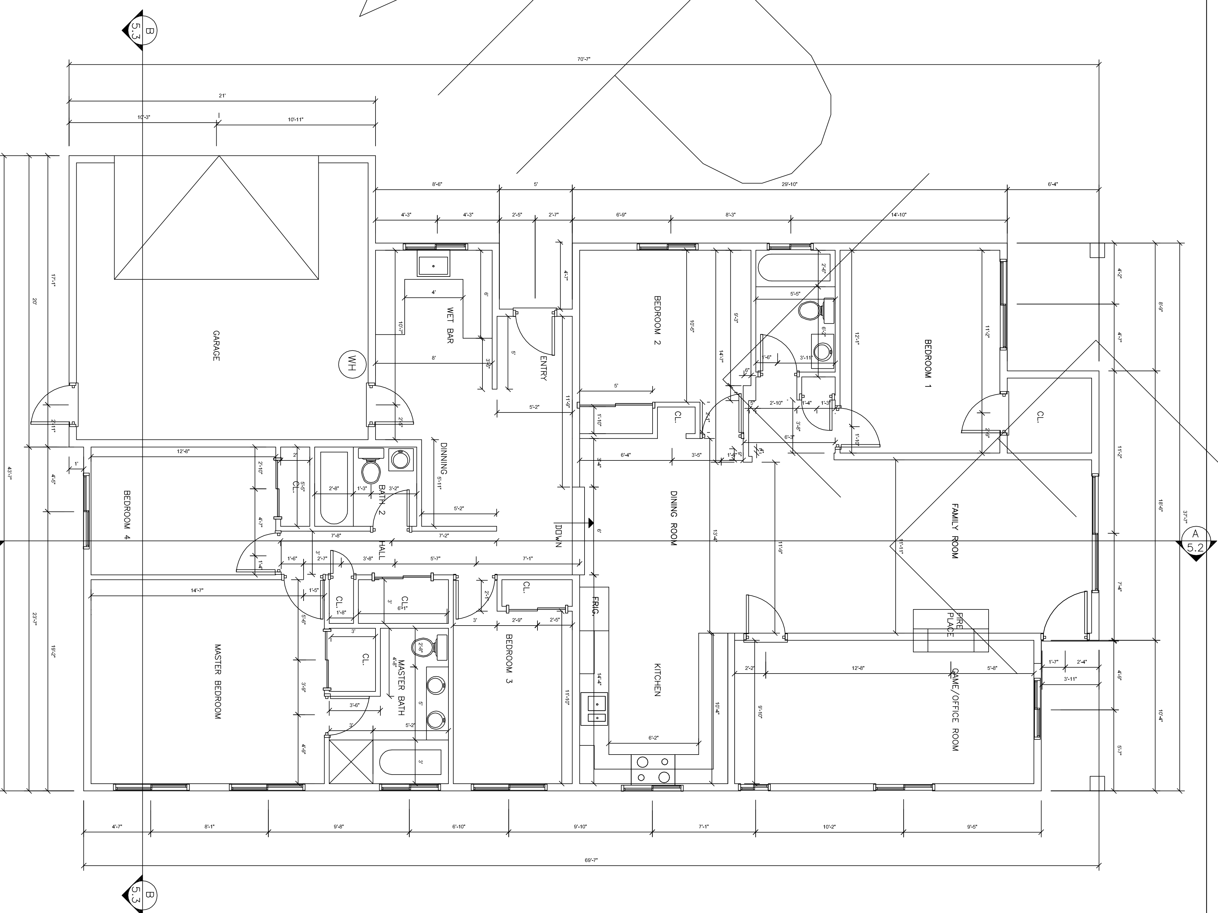
A-1.2 NEW FLOOR PLANS WITH DIMENSIONS
